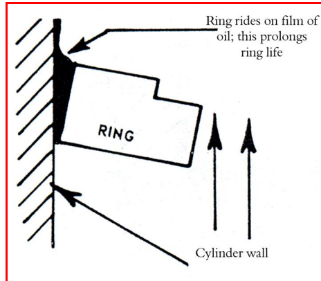
Figure 1.21: On compression and exhaust strokes rings tip and slide easily on a film of oil.
