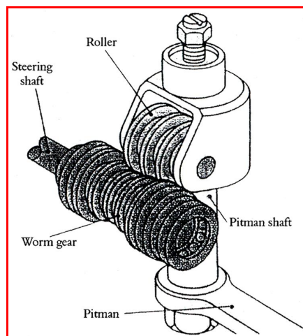
Figure 3.16: Worm and roller gearbox
