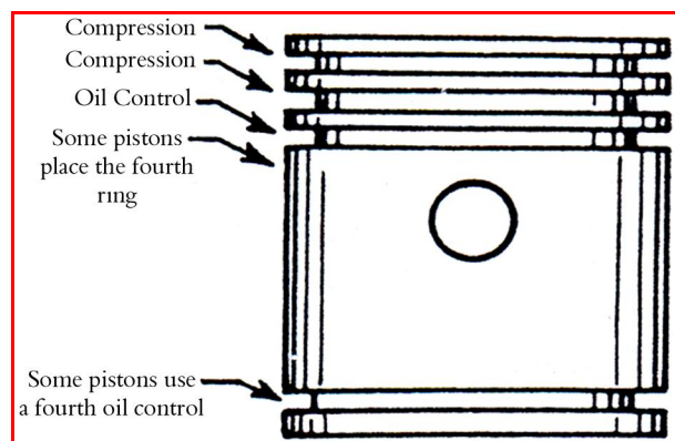
Figure 1.18: Location of compression and oil control rings
