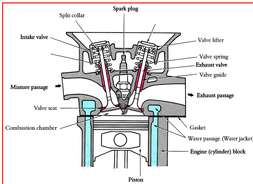
Figure 1.6: Description of each part of cylinder head (cover)
