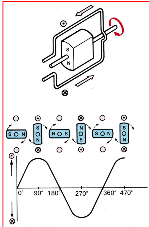
Figure 4.13: Generating alternating current
