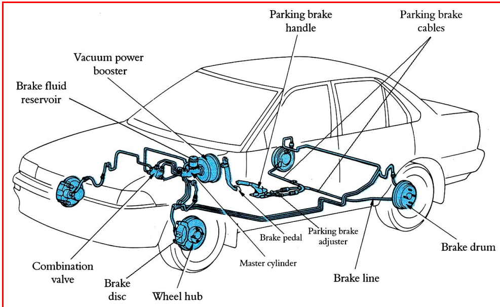
Figure 3.1: A Typical Brake System
