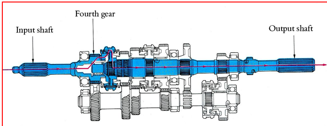
Figure 2.11: Fourth gear position
