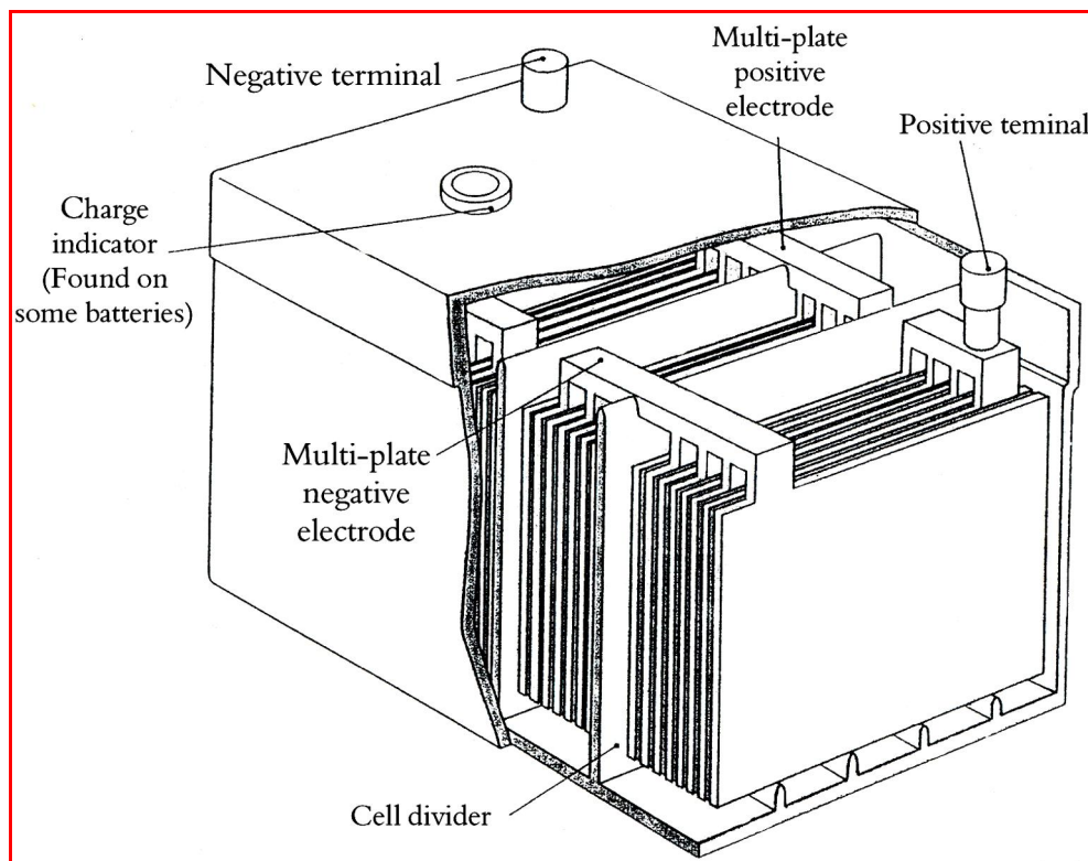
Figure 4.6: Structure of battery
