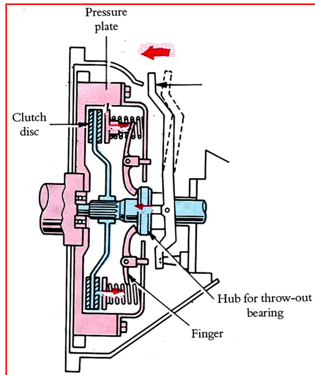
Figure 2.1: Description of the coil-spring clutch
