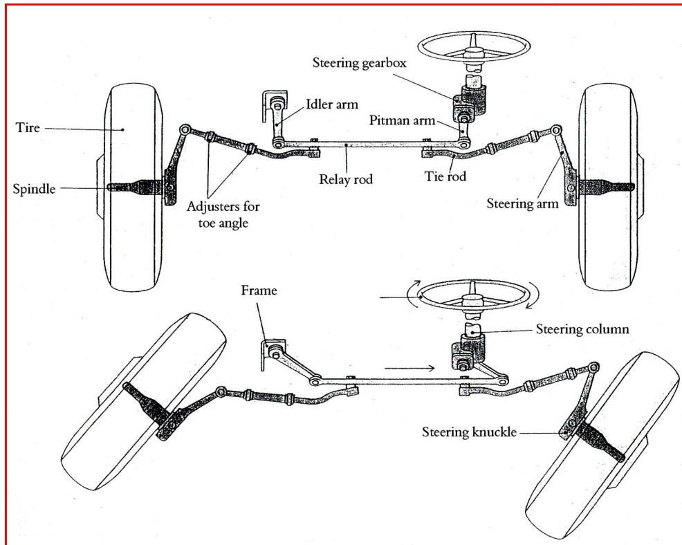
Figure 3.11: Parallelogram steering
