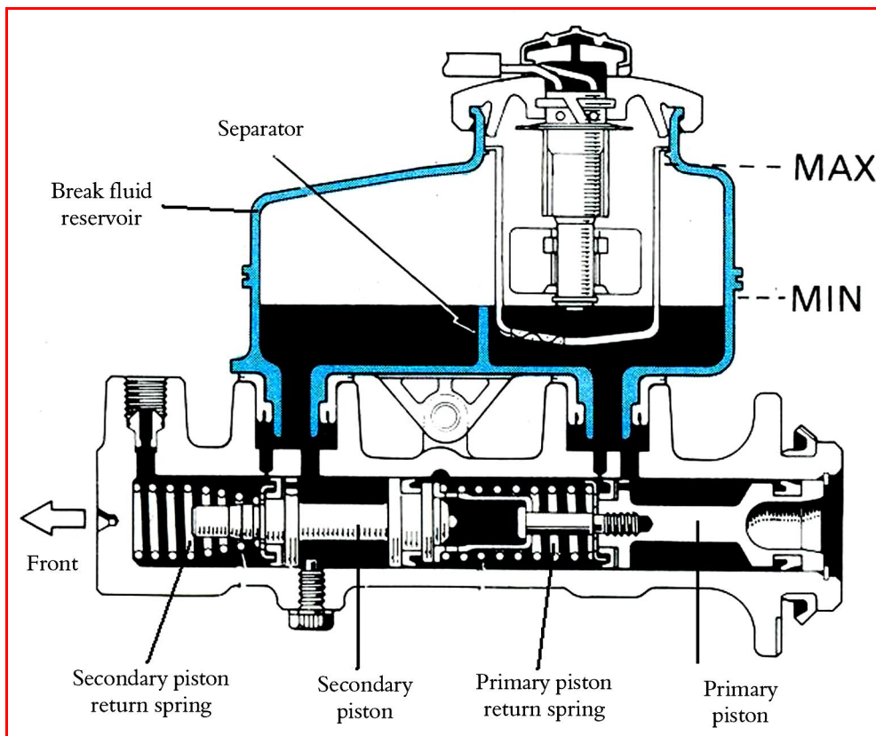
Figure 3.3: Part of master piston
