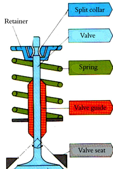
1.28: Parts of valve system
