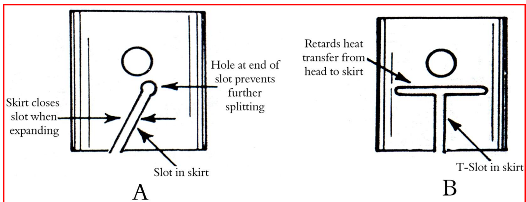
Figure 1.10: Split skirt and T-slot
