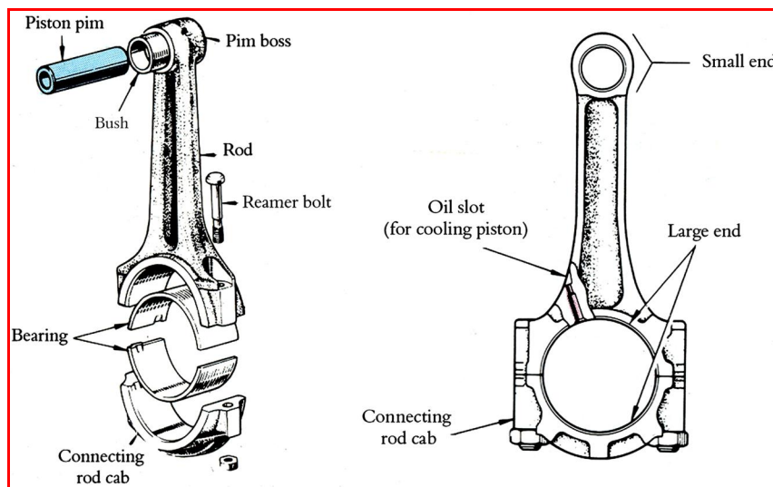
Figure 1.11: Description of each part of connecting rod
