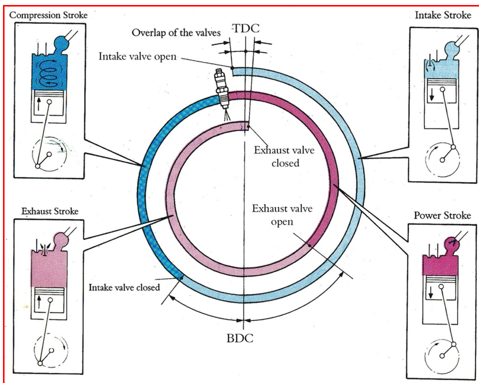
Figure 1.33: Running principle of the four-cylinder diesel engine
