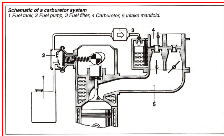
Figure 1.43: Schematic of a carburetor system
