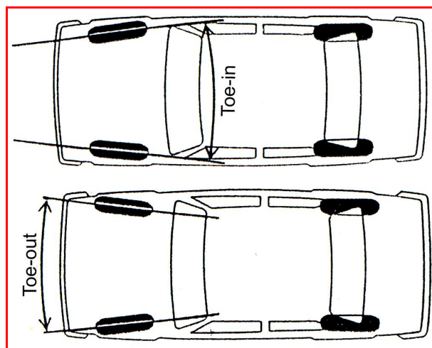
Figure 3.24: Toe-in and toe-out
