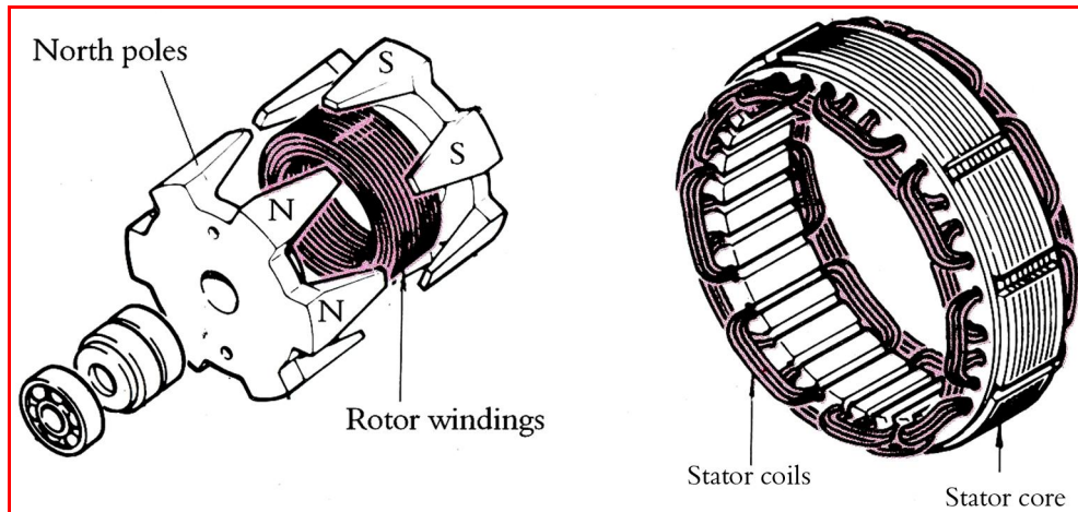
Figure 4.12: Rotor and stator
