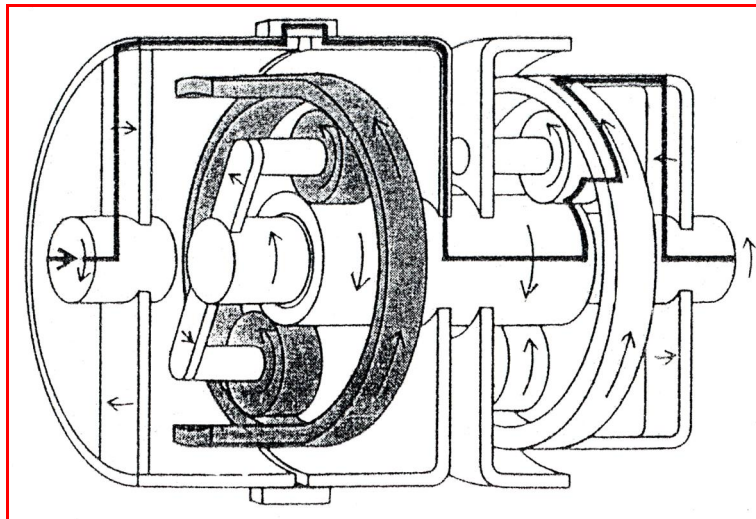
Figure 2.18: Reverse gear
