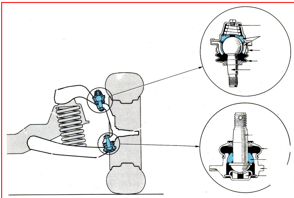
Figure 3.27: Types of ball joints
