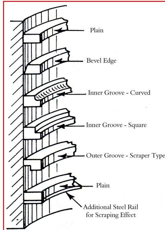
Figure 1.19 Typical compression ring shape, as they would look in a cylinder
