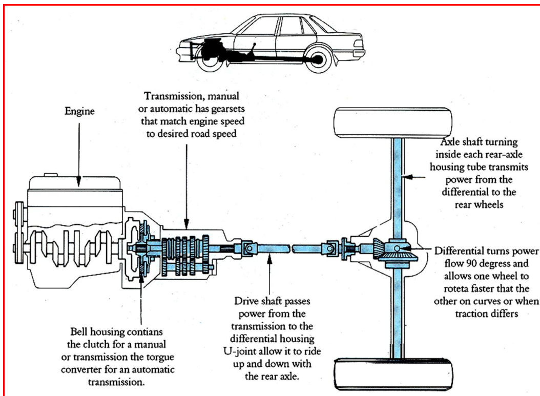
Figure Power Transfer Parts of Front-wheel Drive
