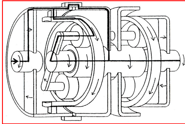
Figure 2.17: High gear
