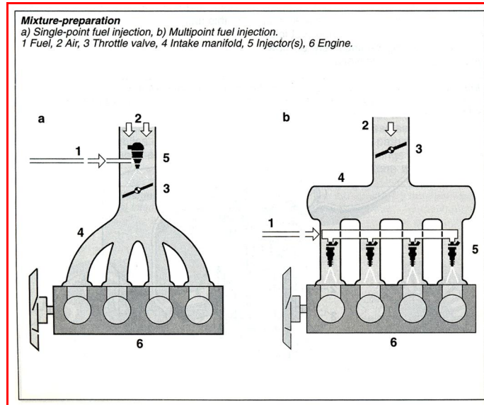
Figure 1.42: Mixture-Preparation
