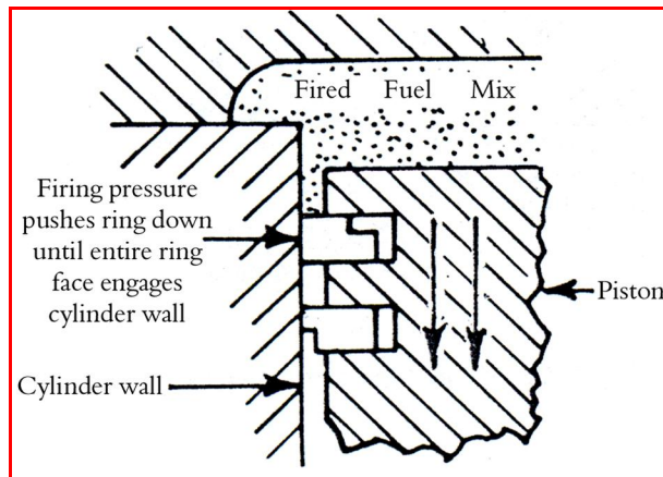
Figure 1.22 Firing pressure forces ring face against wall to provide a good seal
