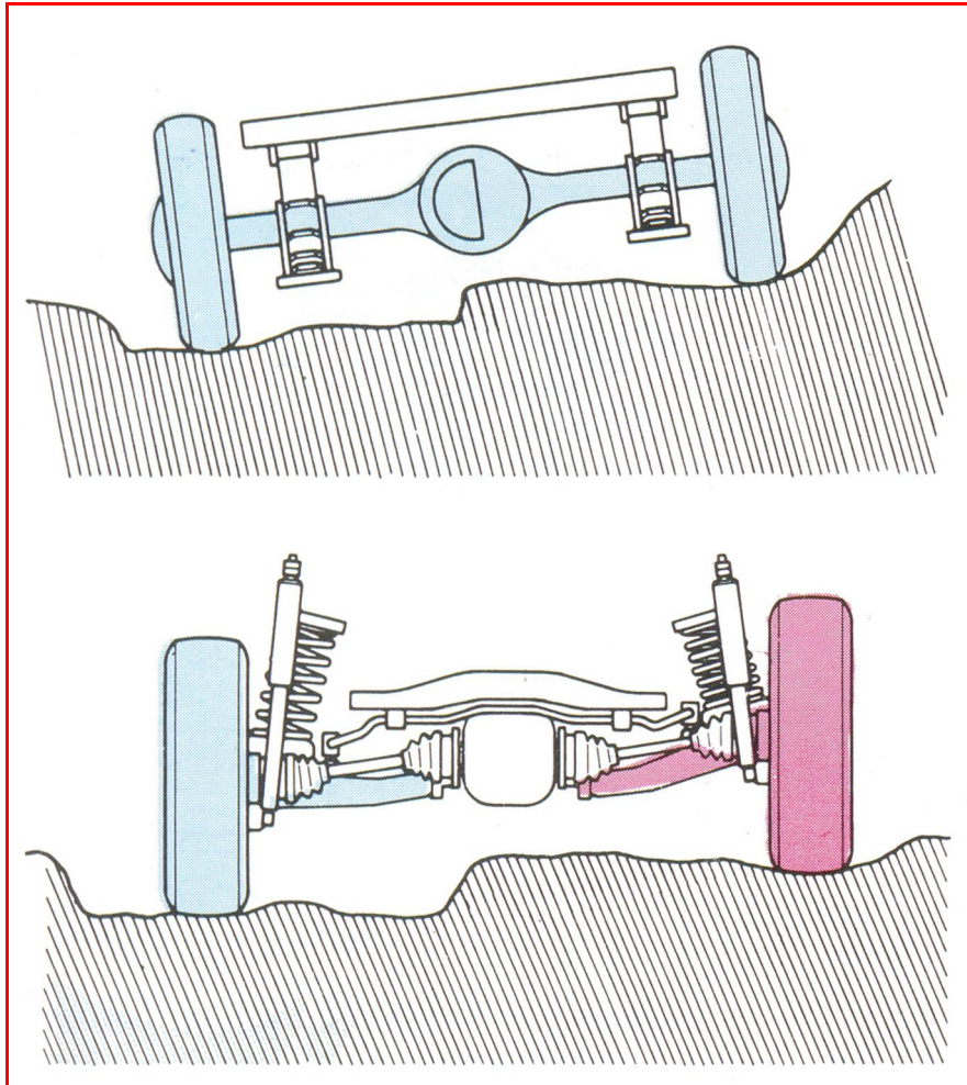
Figure3.25: Types of suspension systems
