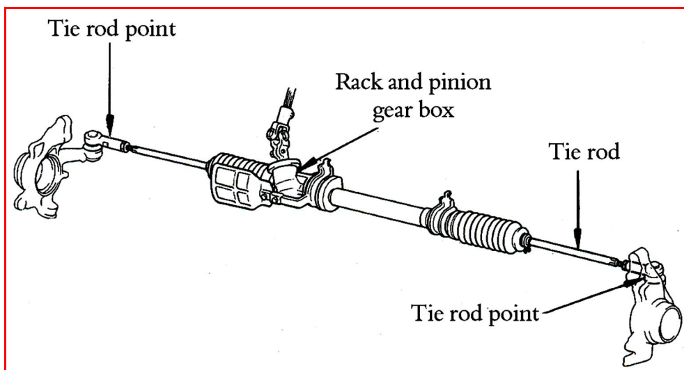
Figure 3.14: Rack and pinion steering linkage
