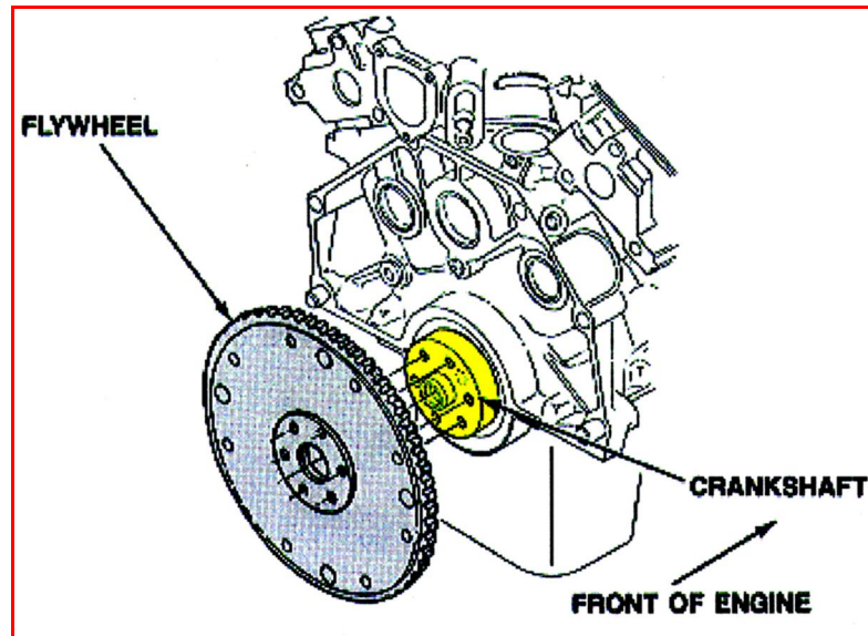
Figure 1.32: Flywheel assemble
