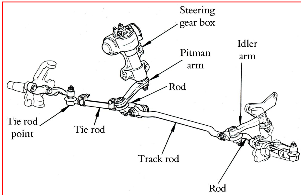
Figure 3.13: Parallelogram steering linkage
