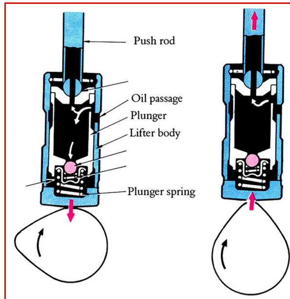
Figure 1.30: Hydraulic lifters
