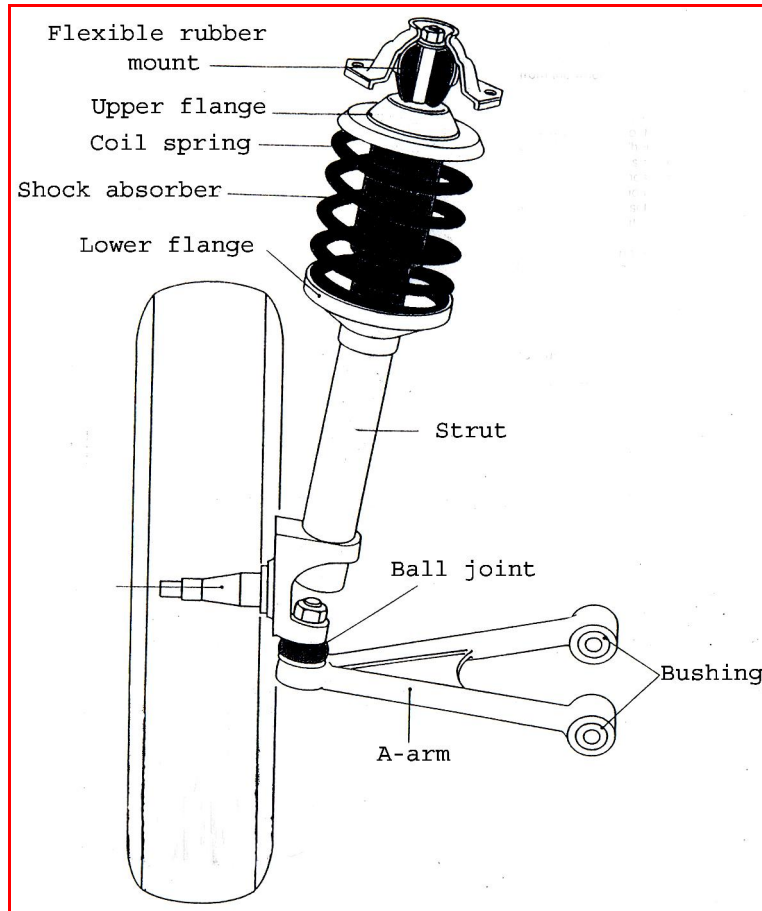
Figure 3.2: Mac Pherson strut system
