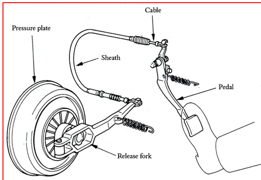
Figure 2.4: Cable operation
