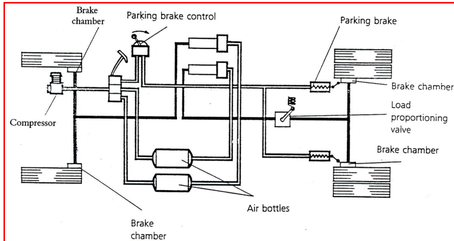
Figure 3.4: Air-hydraulic actuated
