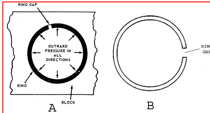
Figure 1.16: Top view of cylinder shows sealing action of piston ring
