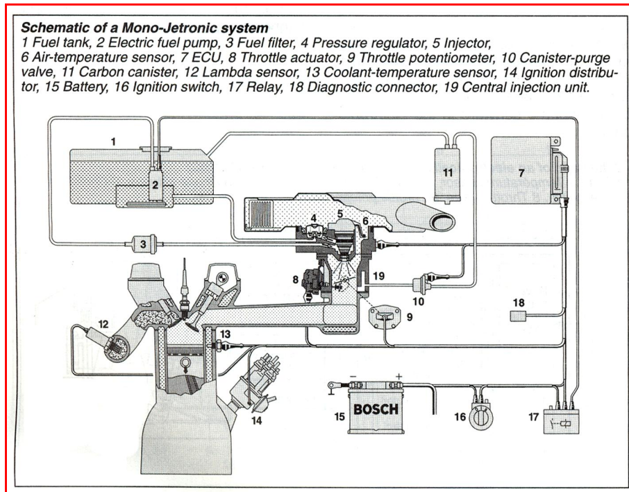
Figure 1.44: Schematic of a Mono-Jetronic system
