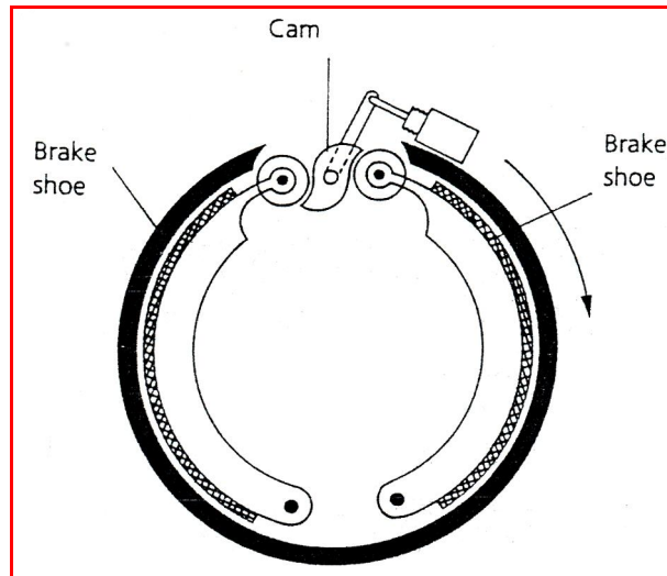
Figure 3.6: Drum brake, cam actuated (simplex)
