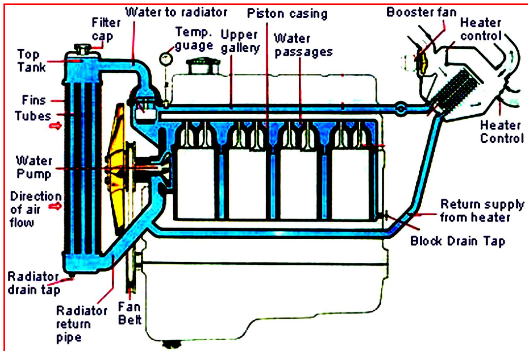
Figure 1.36: Water cooling system
