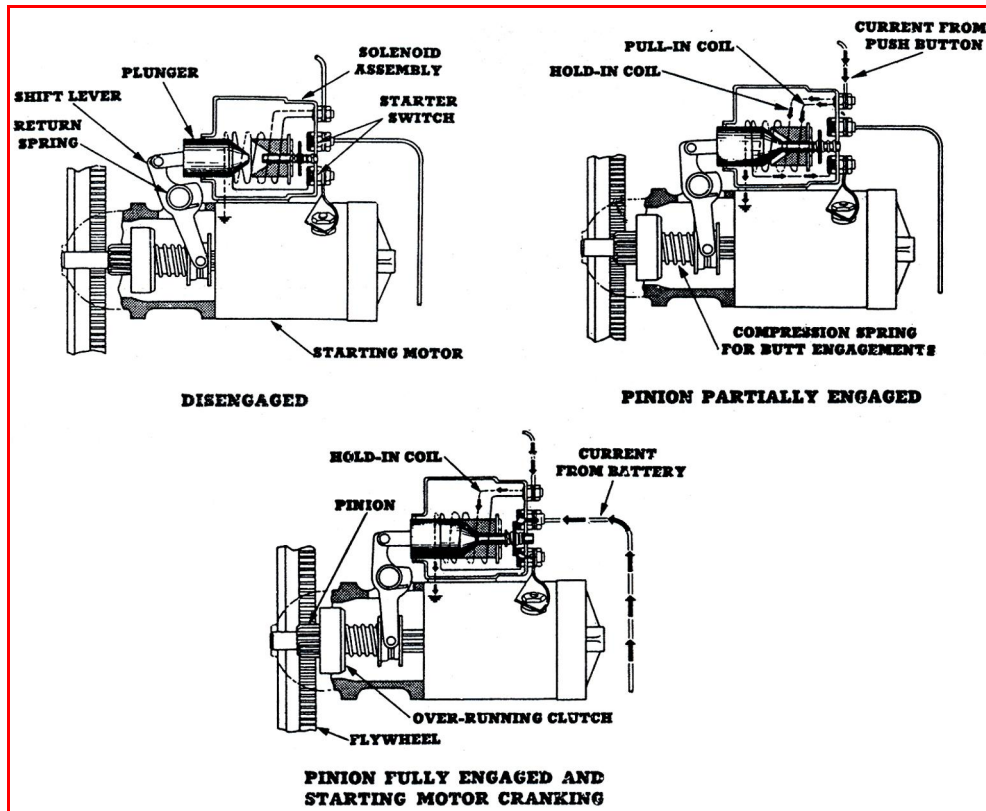
Figure 4.10: Electric solenoid operation
