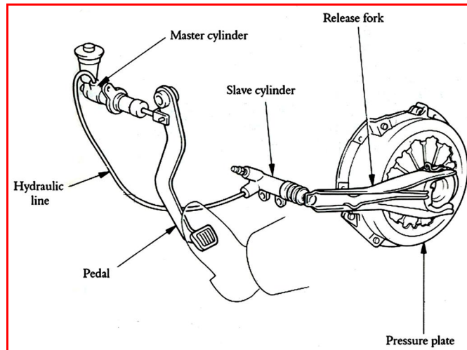
Figure 2.3: Hydraulic operation
