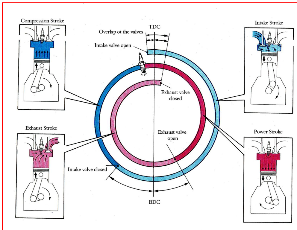
Figure 1.34: Running principle of the four-cylinder Otto (gasoline) engine
