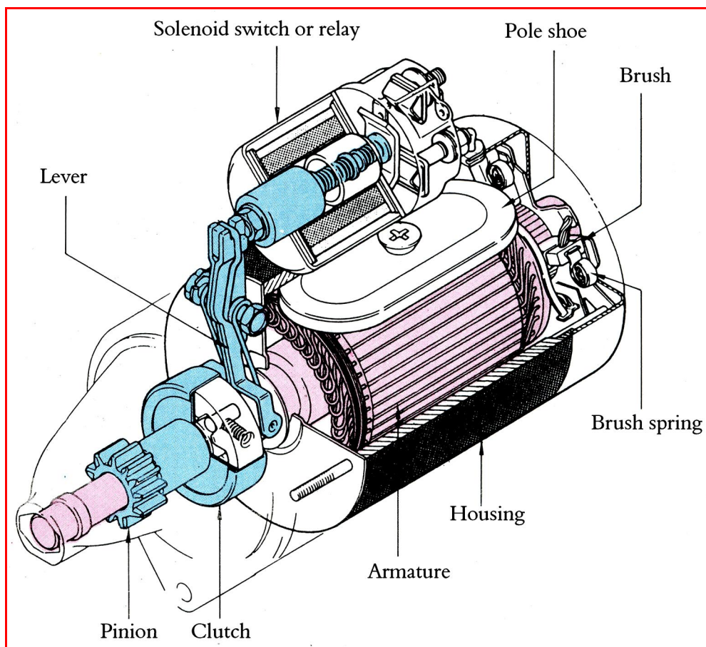
Figure 4.9: Structure of starter
