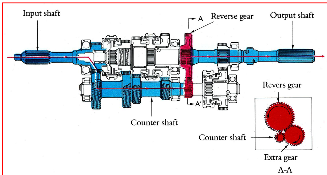
Figure 2.12: Reverse gear position
