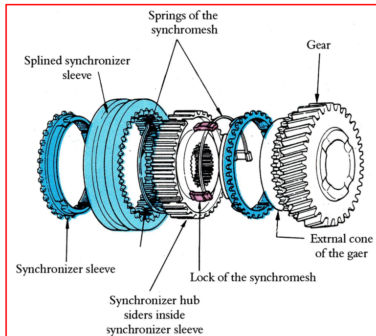
Figure 2.13: Description of the synchromesh system
