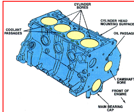
Figure 1.5: In-line four-cylinder engine (cylinder) block
