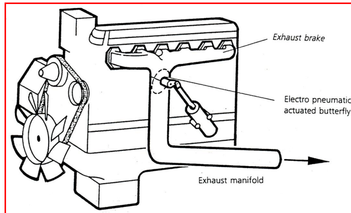
Figure 3.9: Exhaust brake
