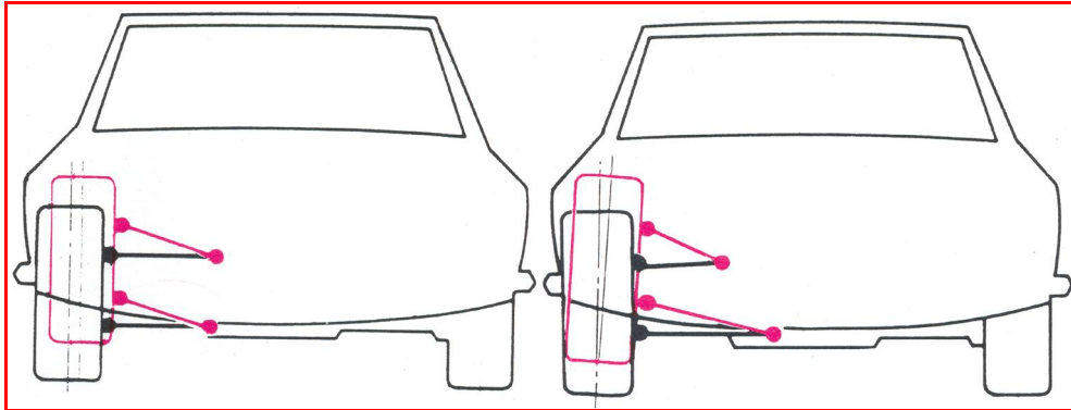
Figure 3.26: Upper and lower A-arms
