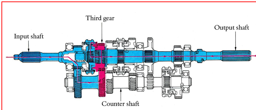
Figure 2.10: Third gear position
