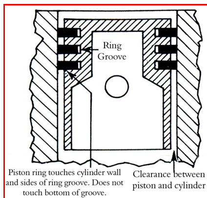
Figure 1.15: Piston rings seal gap between piston and cylinder wall
