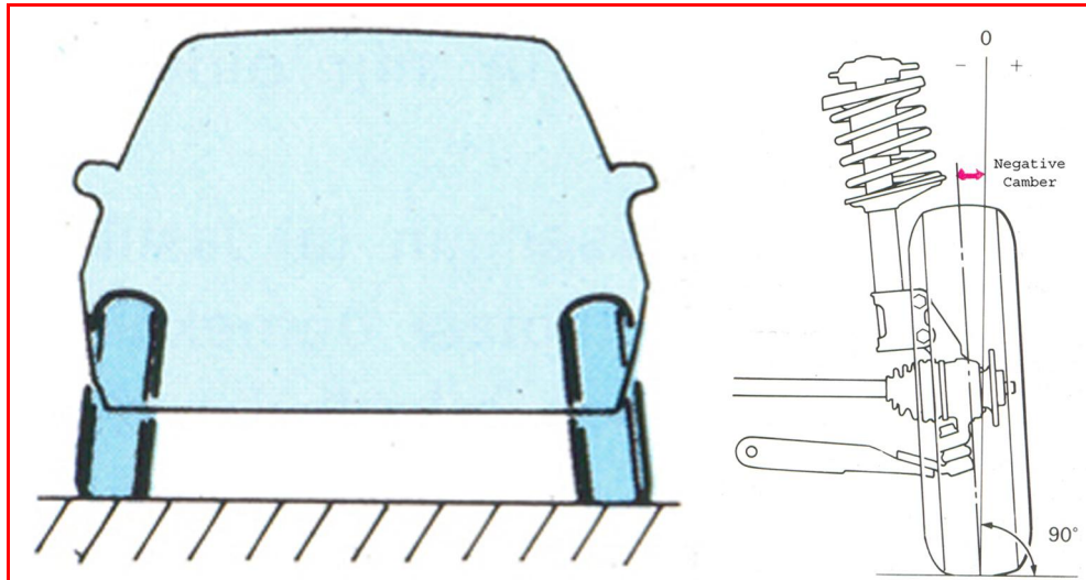
Figure 3.20: Negative camber
