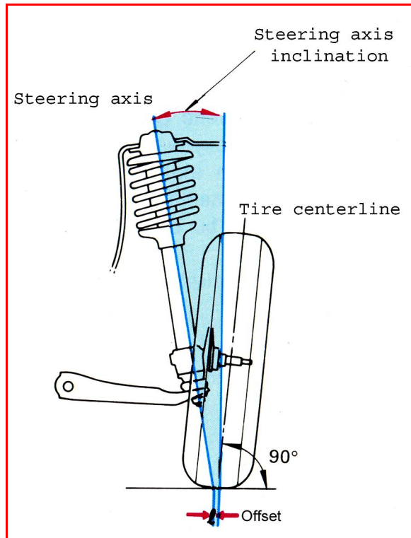
Figure 3.23: Steering axis inclination
