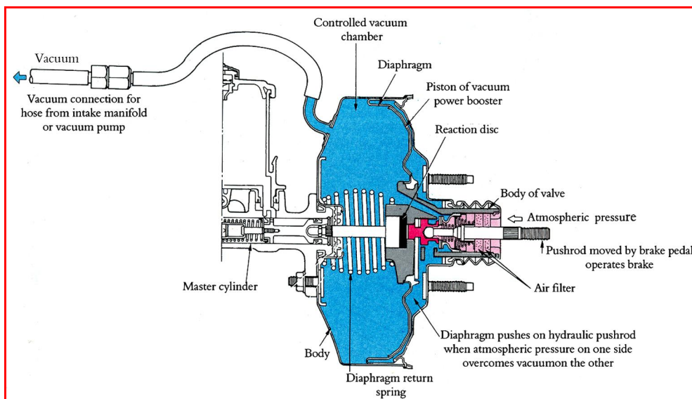
Figure 3.2: Vacuum power booster assembly
