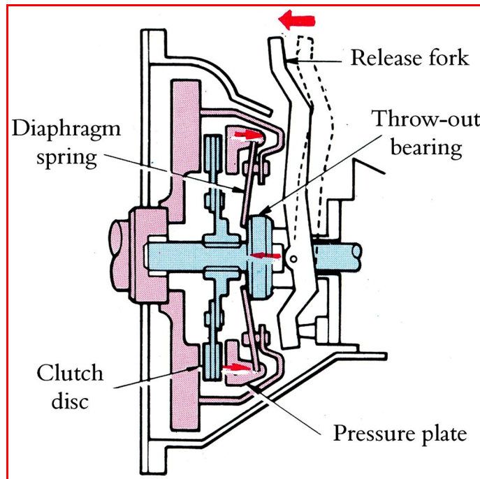
Figure 2.2: Description of the spring clutch
