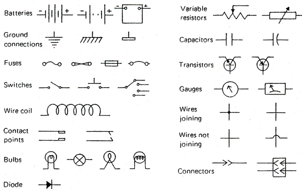
Figure 4.5: Electrical symbols
