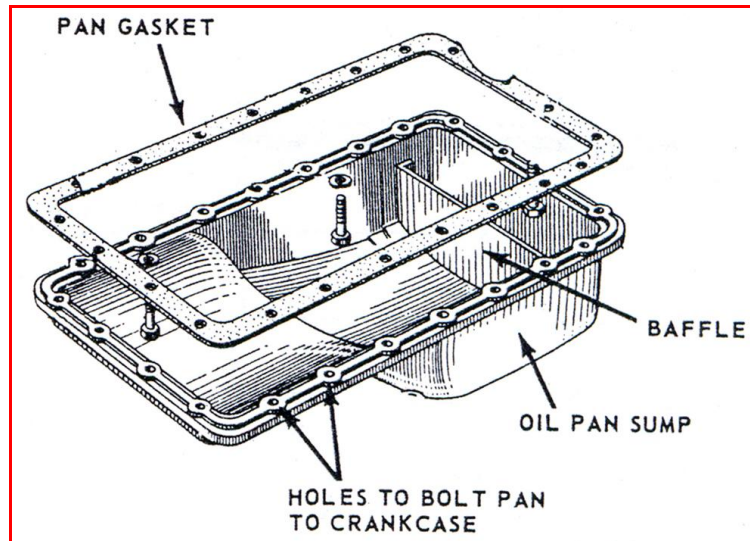
Figure 1.7: Oil pan
