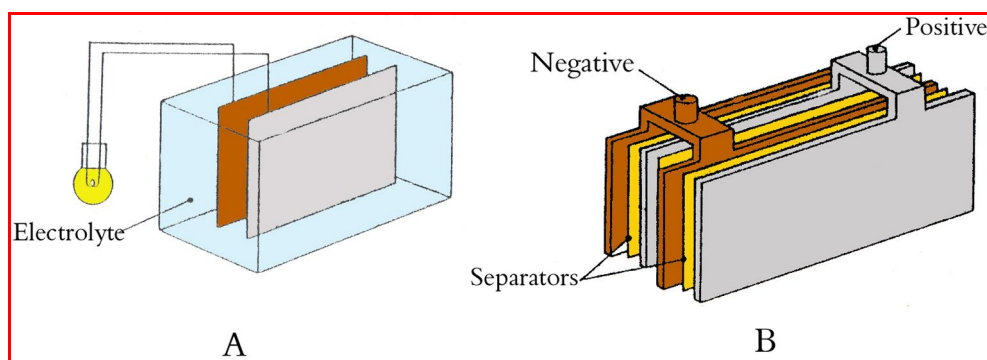
Figure 4.7: Create electric energy into battery
