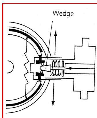
Figure 3.7: Drum brake, wedge actuated (simplex)
