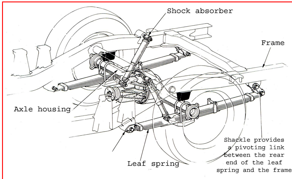
Figure 3.31: Hotchkiss suspension system
