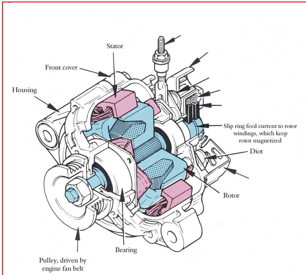
Figure 4.11: Structure alternator
