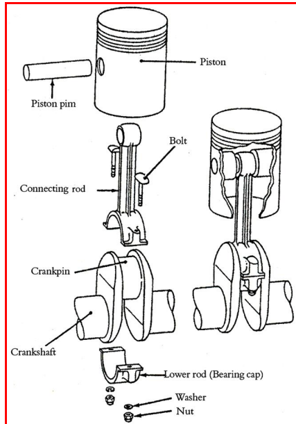
Figure 1.13: Connecting piston and connecting rod
