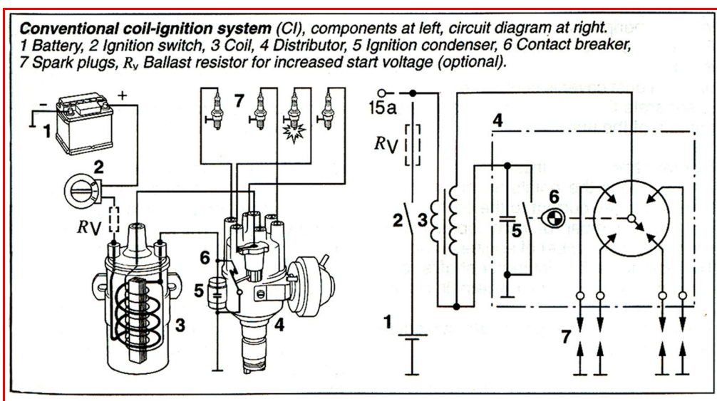
Figure 1.38: Conventional Coil-Ignition System
