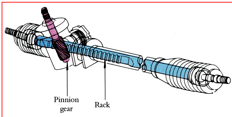
Figure 3.15: Rack and pinion gearbox
