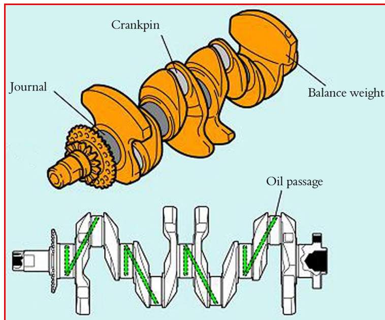
Figure 1.26: Parts of crankshaft
