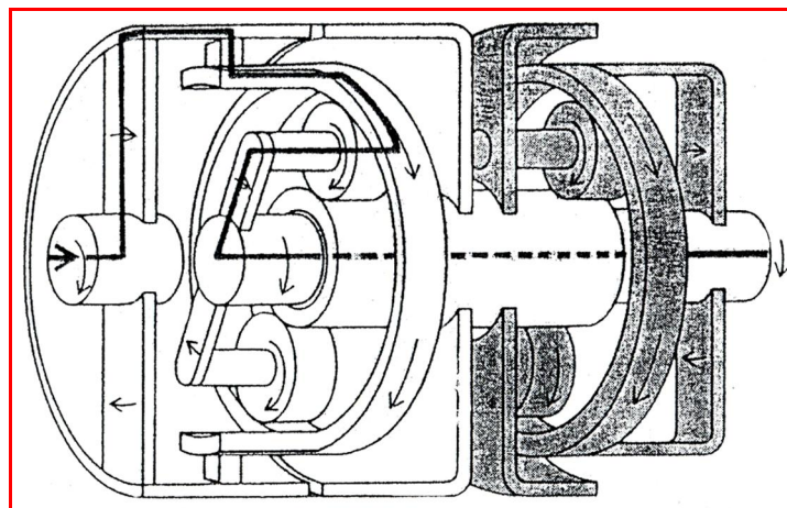
Figure 2.16: Second gear
