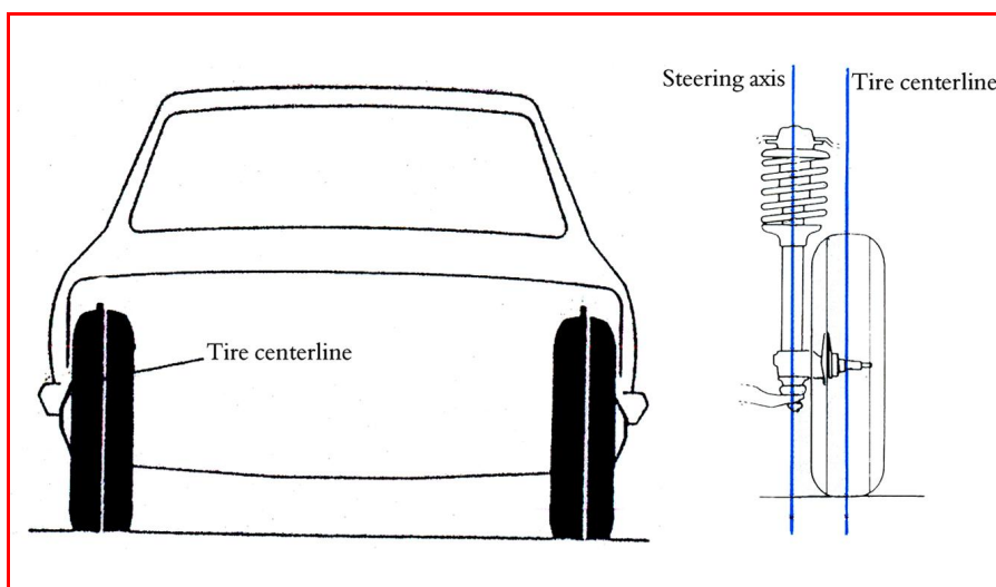
Figure 3.19: Zero camber
