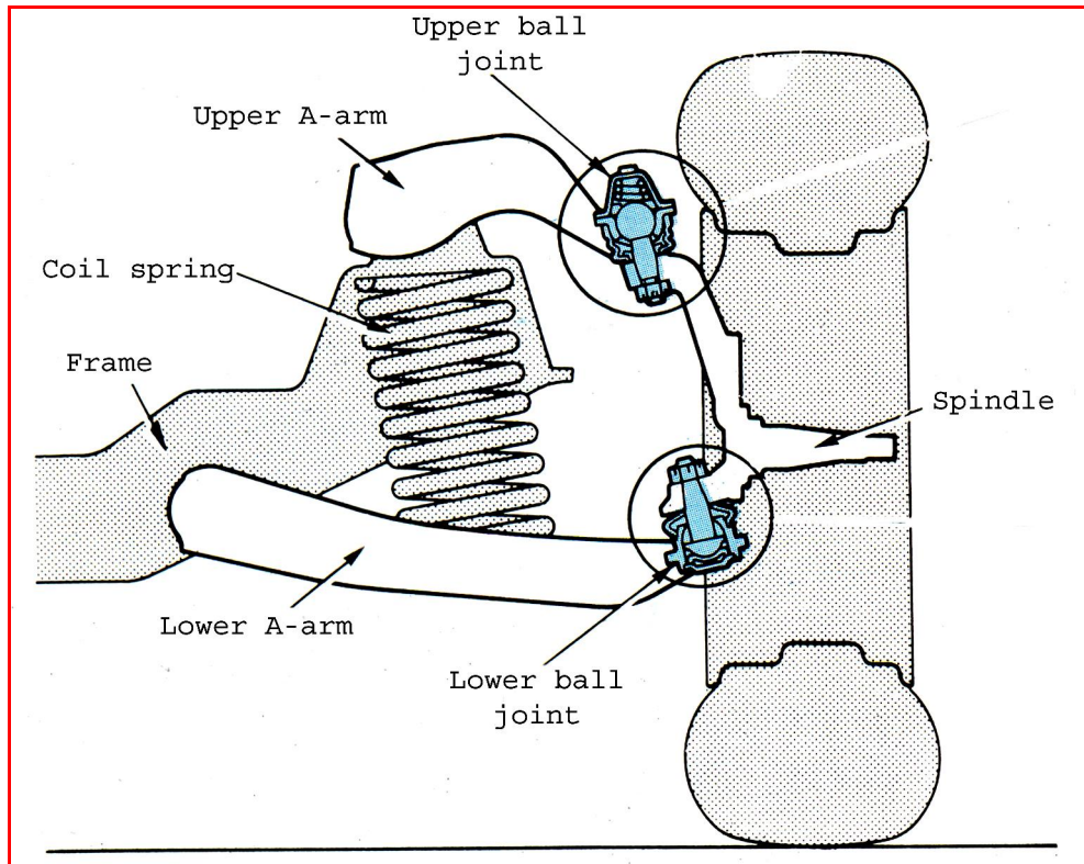
Figure 3.28: Part of double A-arm suspension system
