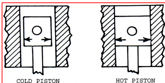
Figure 1.9: Exaggerated view shows effect of heat on piston expansion.
