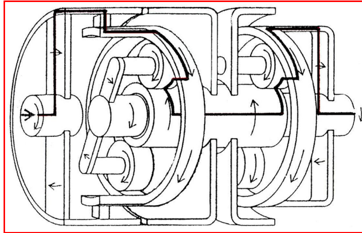
Figure 2.15: First gear
