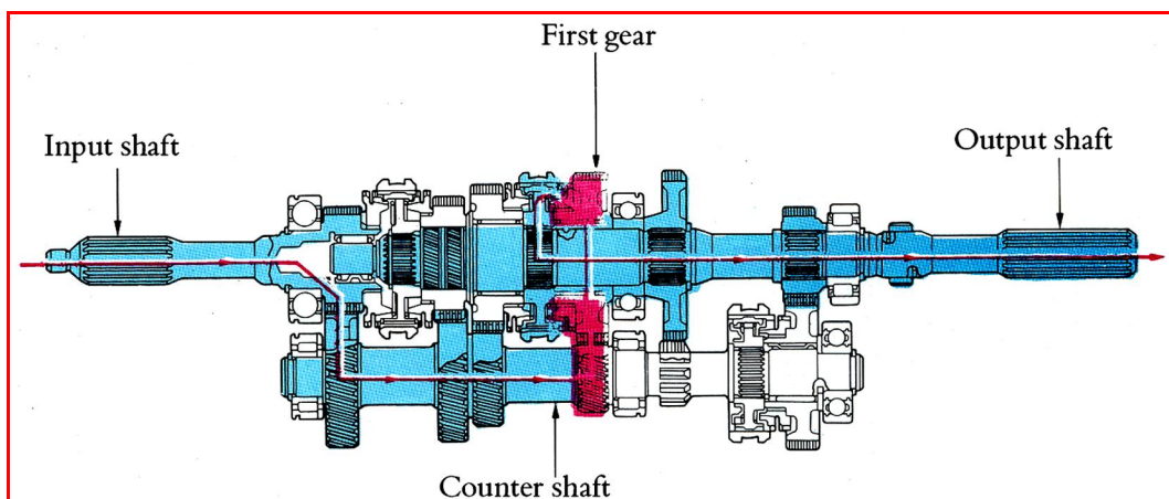
Figure 2.8: First gear position
