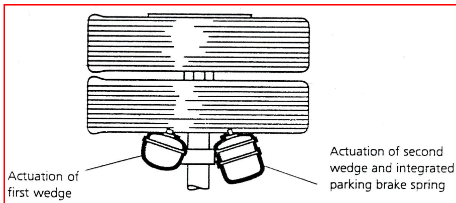
Figure 3.8: Brake chamber. (duo duplex system)
