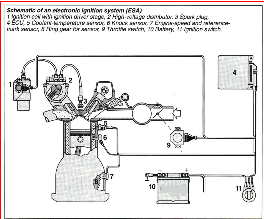
Figure 1.40: Schematic of an electronic ignition system
