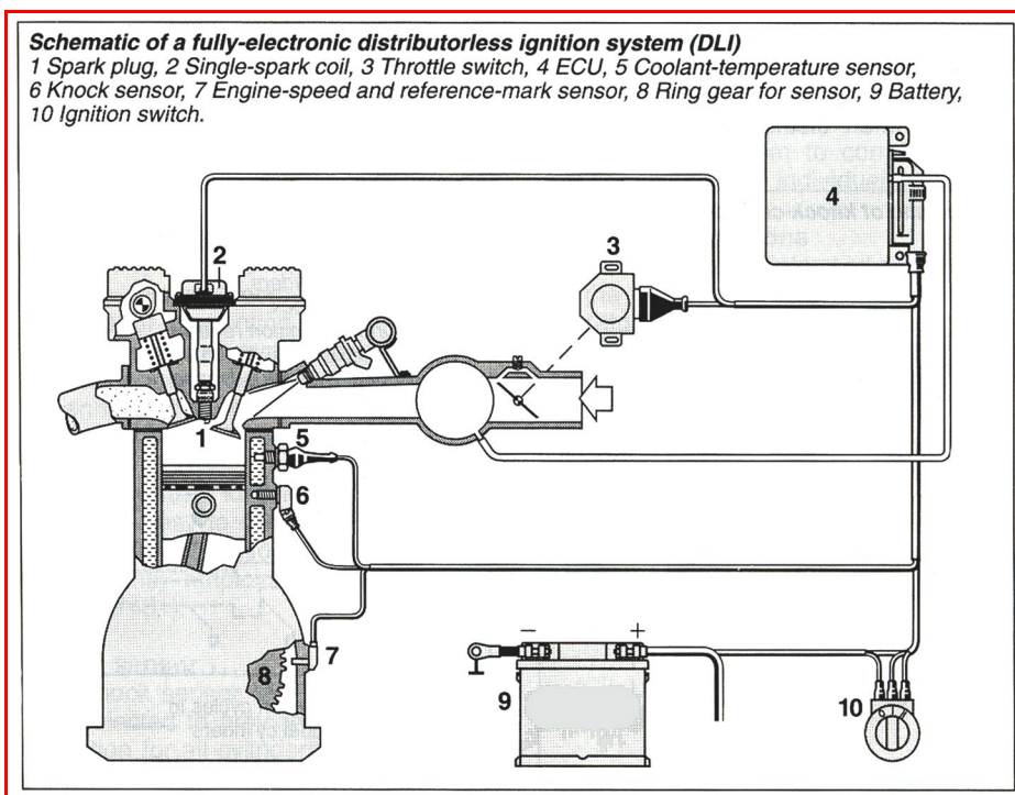
Figure 1.41: Schematic of a fully-electronic distributorless ignition system
