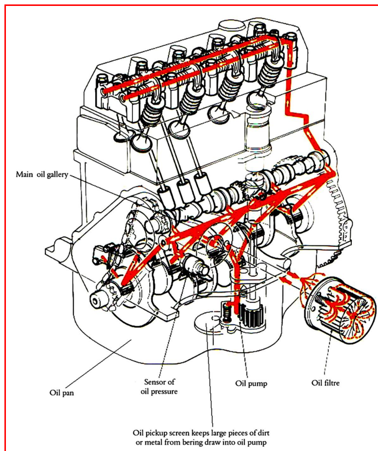
Figure1.35: Passages of lubricating oil
