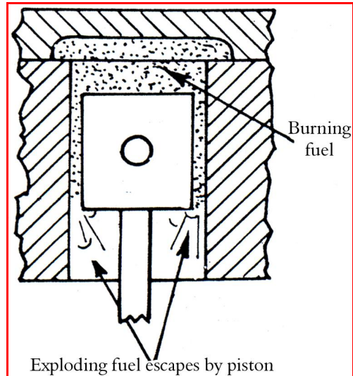
Figure 1.14: Piston cannot seal by itself because clearance with cylinder wall must be maintained
