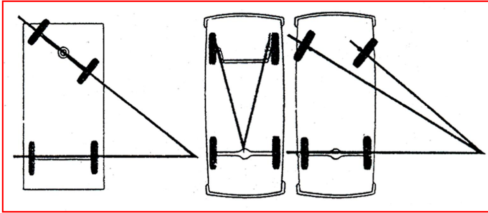
Figure 3.12: Geometrically correct
