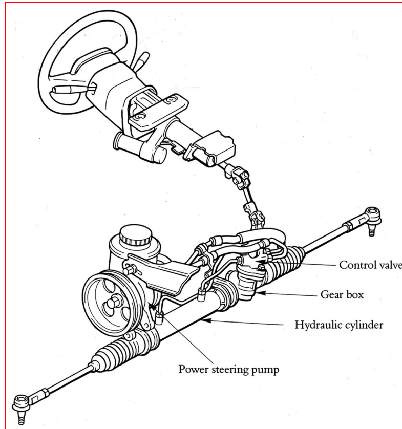
Figure 3.18: Power steering
