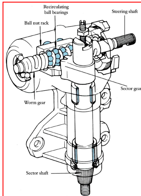
Figure 3.17: Recirculating-ball gearbox
