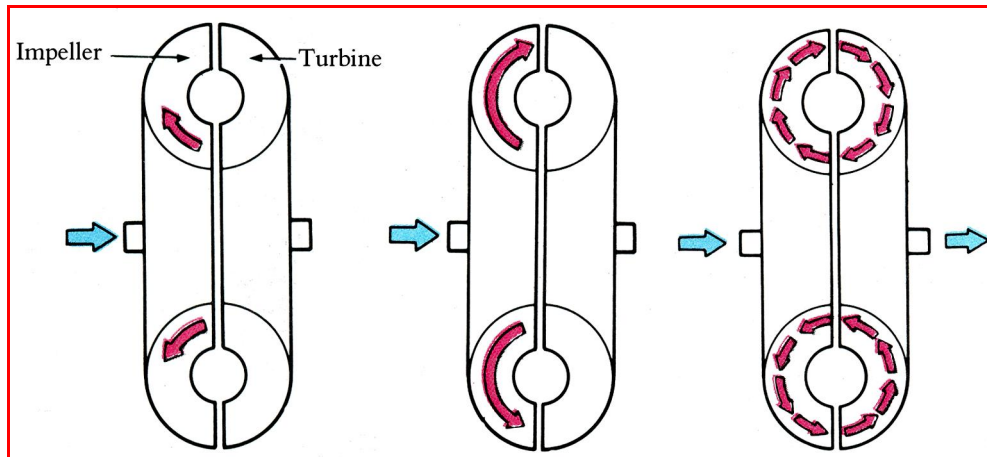
Figure 2.14: Progressive engagement of fluid clutch
