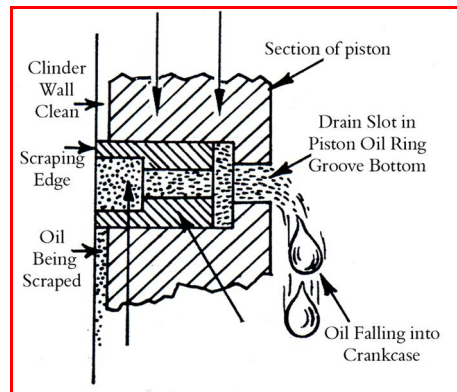
Figure 1.24: Action of oil ring as it travels down cylinder well
