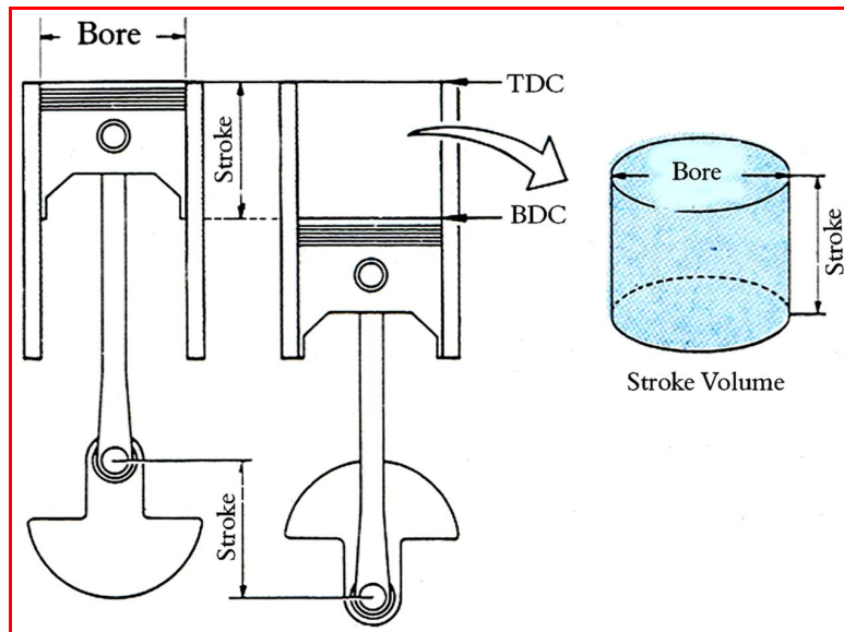
Figure 1.2: Stroke and Stroke Volume
