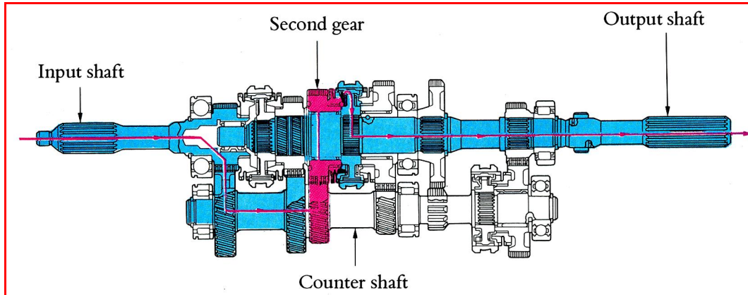
Figure 29: Second gear position
