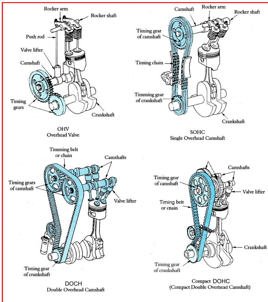
Figure 1.27: The type of valve mechanism
