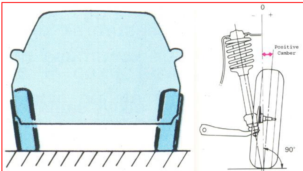
Figure 3.21: Positive Camber
