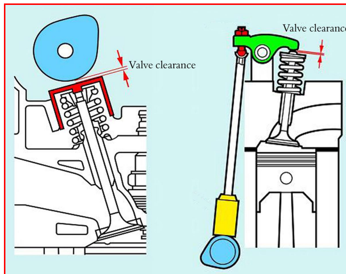
Figure 1.31: Valve clearance
