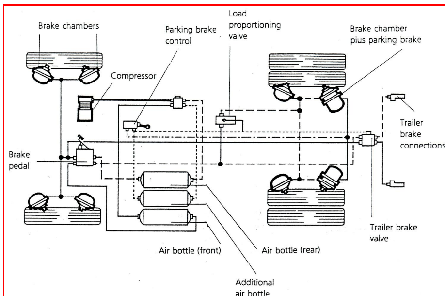
Figure 3.5: Fully pneumatic brake system
