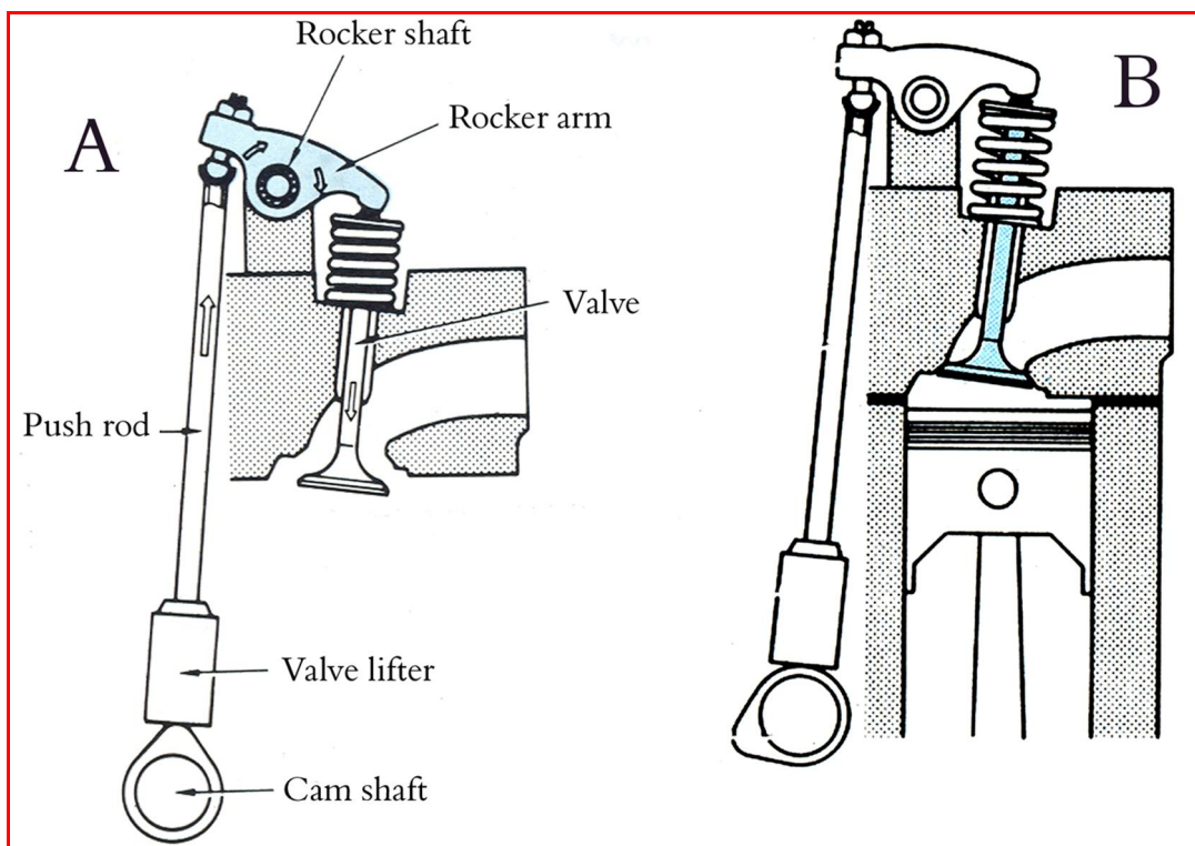
Figure 1.29: Valve operation
