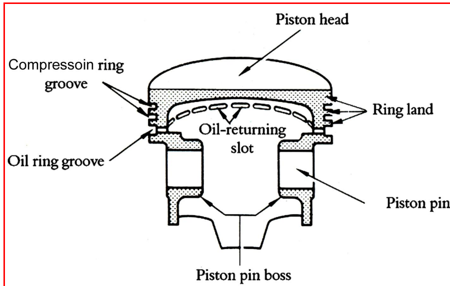
Figure 1.8: Description of each part of piston
