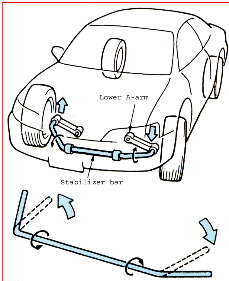
Figure 3.30: Stabilizer bar
