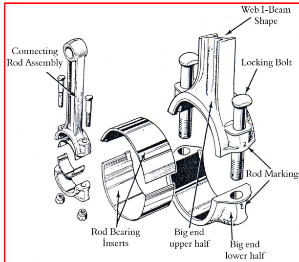
Figure 1.12: Typical connecting rod construction
