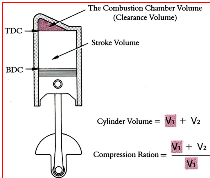
Figure 1.3: The Combustion Chamber Volume and Compression Ratio
