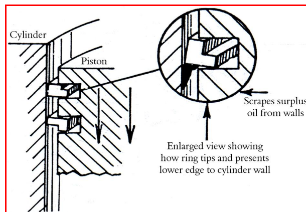
Figure 1.20 Internal stress causes rings to tip and act as mild scrapers
