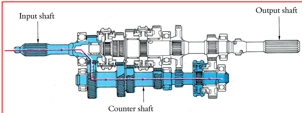
Figure 2.7: Neutral position
