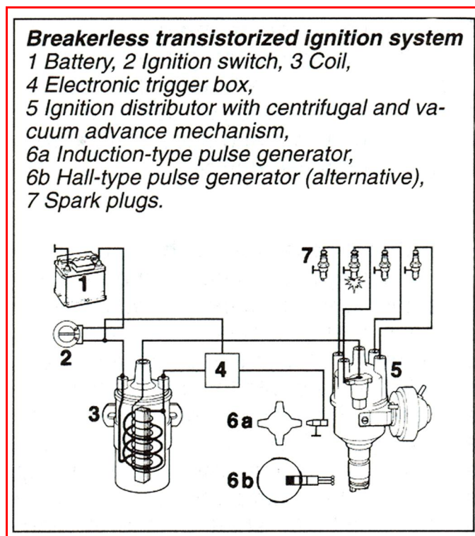
Figure 1.39: Breakerless Transistorized Ignition System
