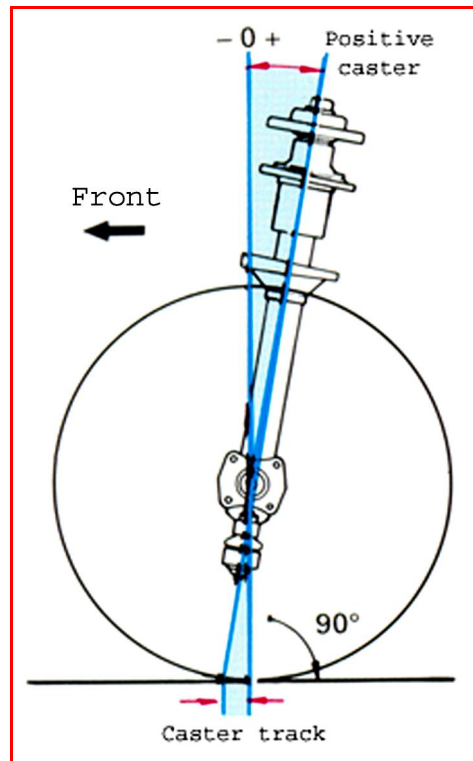
Figure 3.22 Positive caster
