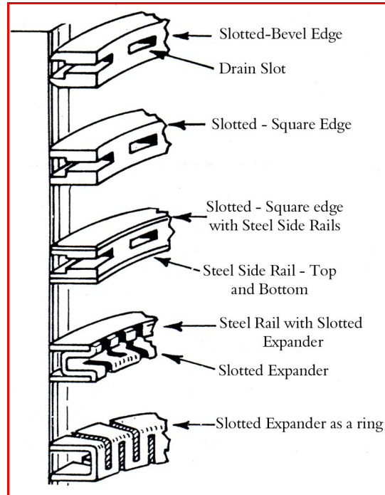
Figure 1.23: Common types of oil control rings
