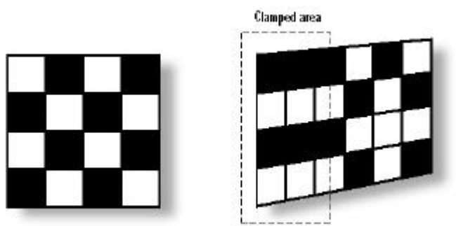
Figure 12-3 GL_CLAMP textures
