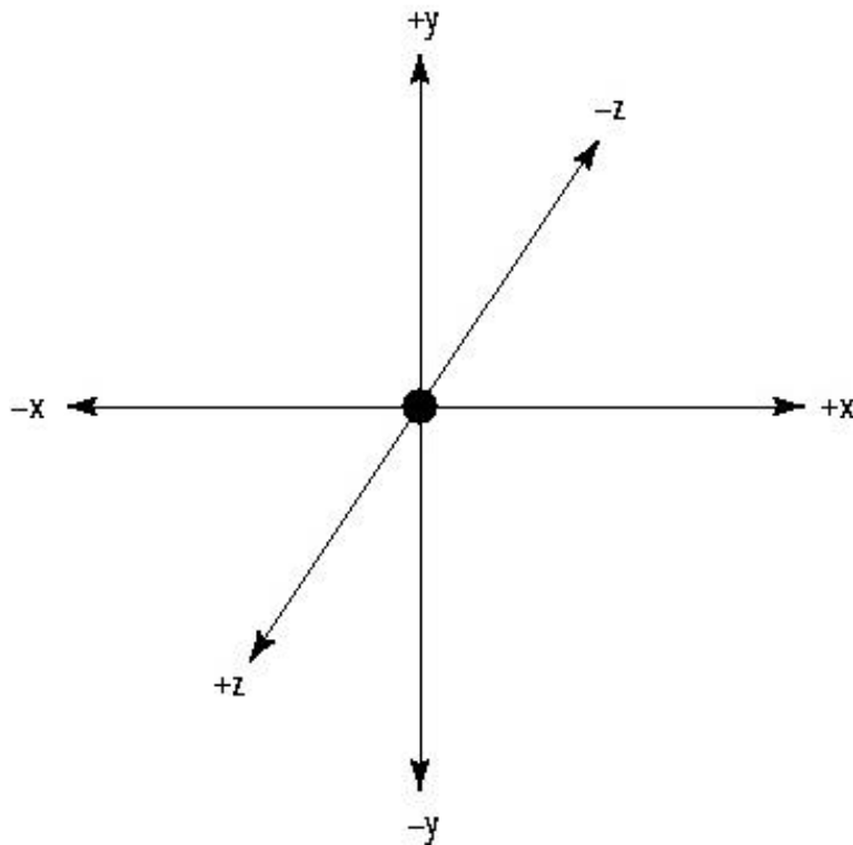
Figure 3-9 Cartesian space
